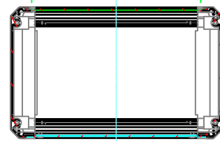
ねじ止めパネル有効寸法 / Screwed panel Max dim. W-46
